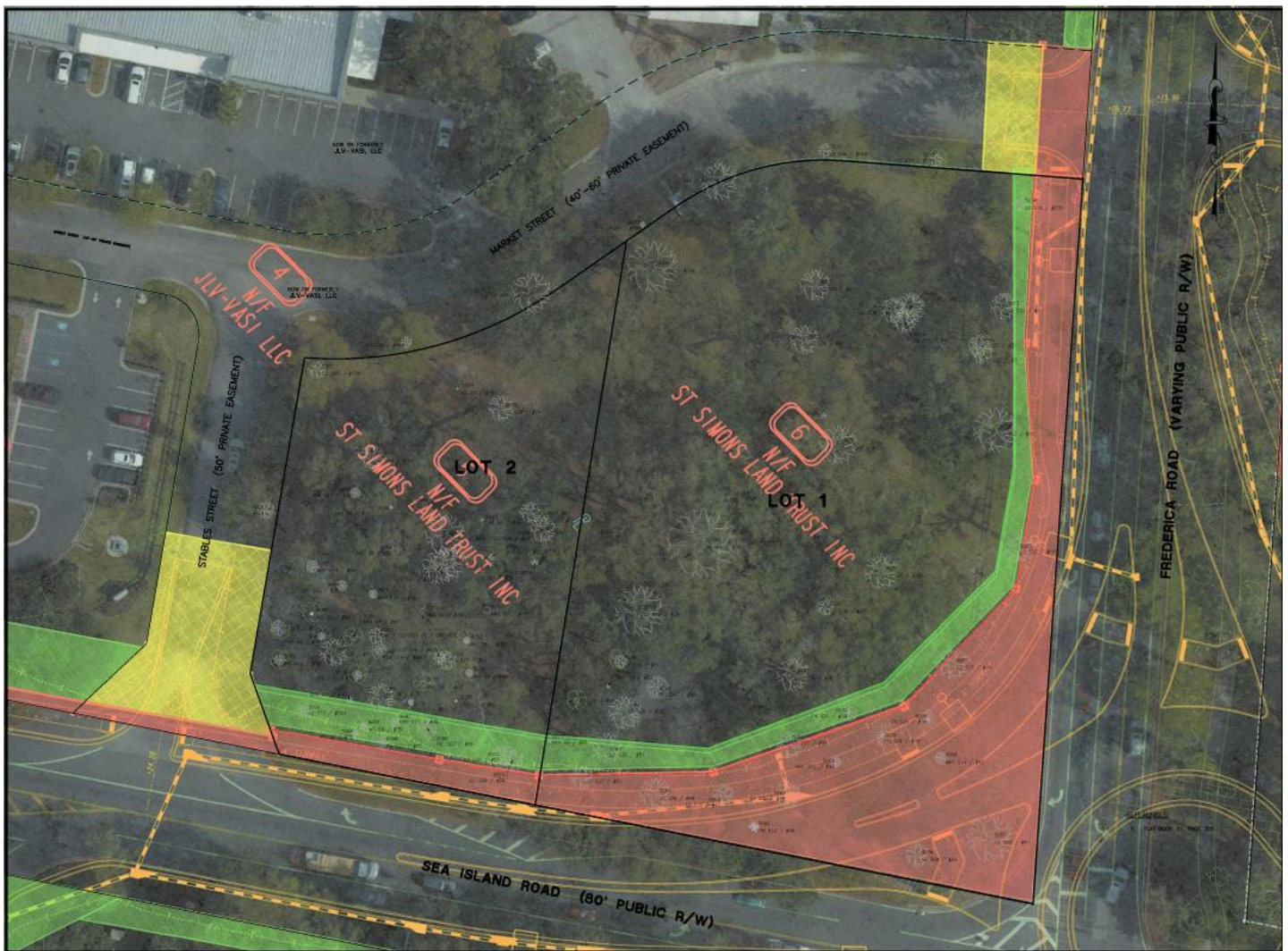
Old Stables Corner Tree Survey Overlayed on Glynn County's "Sea Island at Frederica Right of Way Layout" from Southeastern Engineering, Inc.
